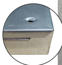
Wrap Around Tray Forming Encapsulation Pre-drilled Holes for Screw Fixing
